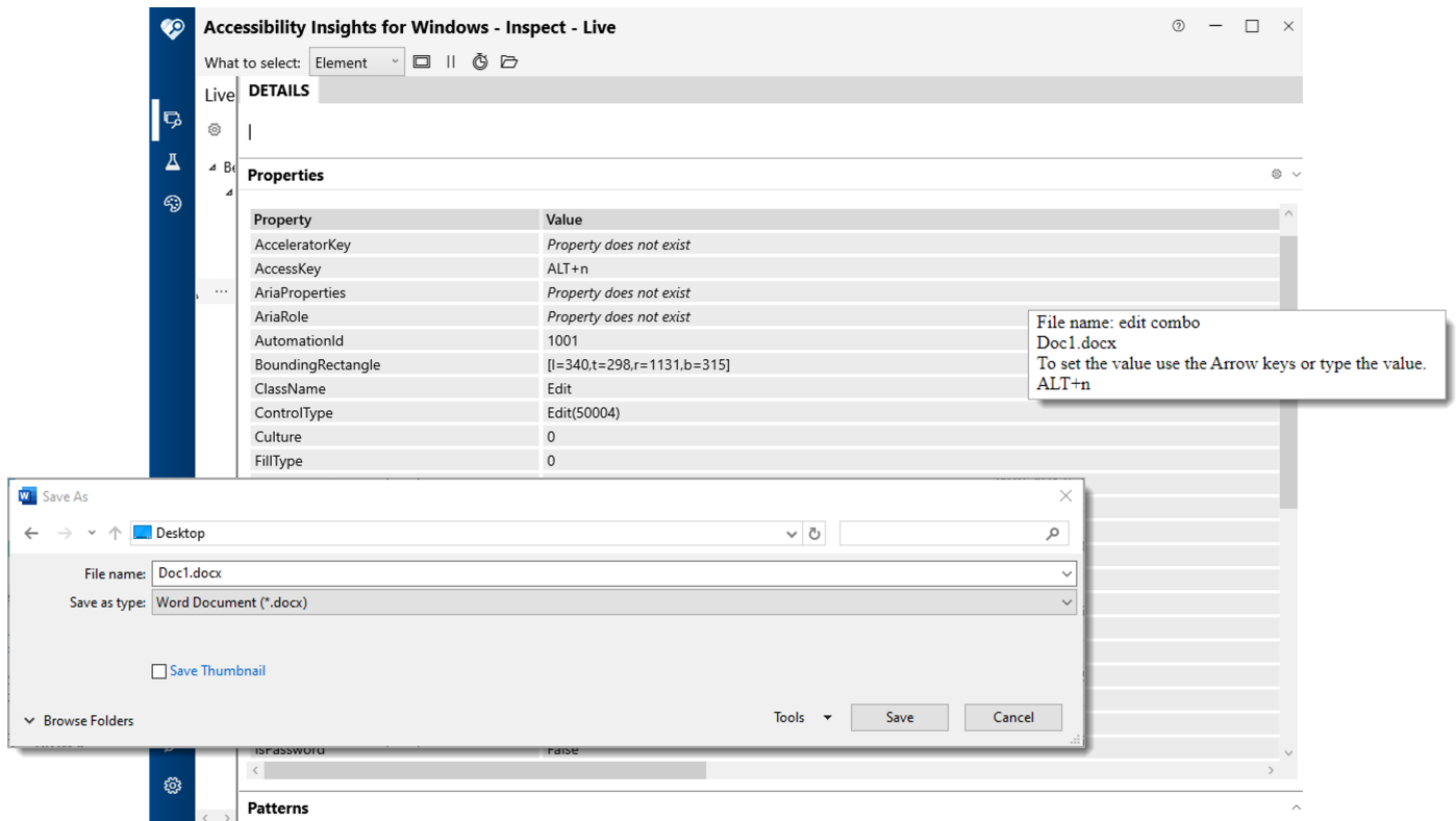
Figure 1: Information of the Accessibility API and its use by the screen reader JAWS
